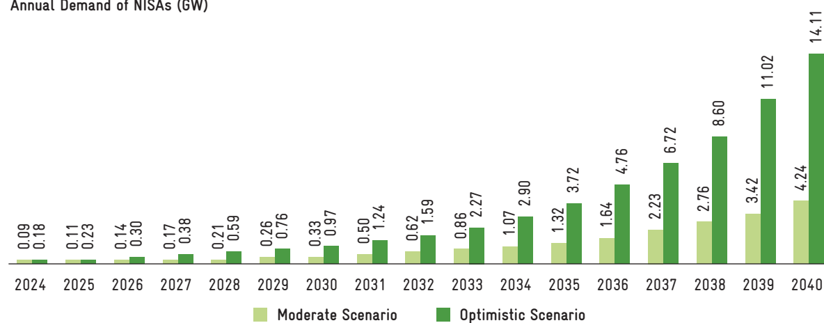
Figure 19: Capacity projections of APV from 2024-40
